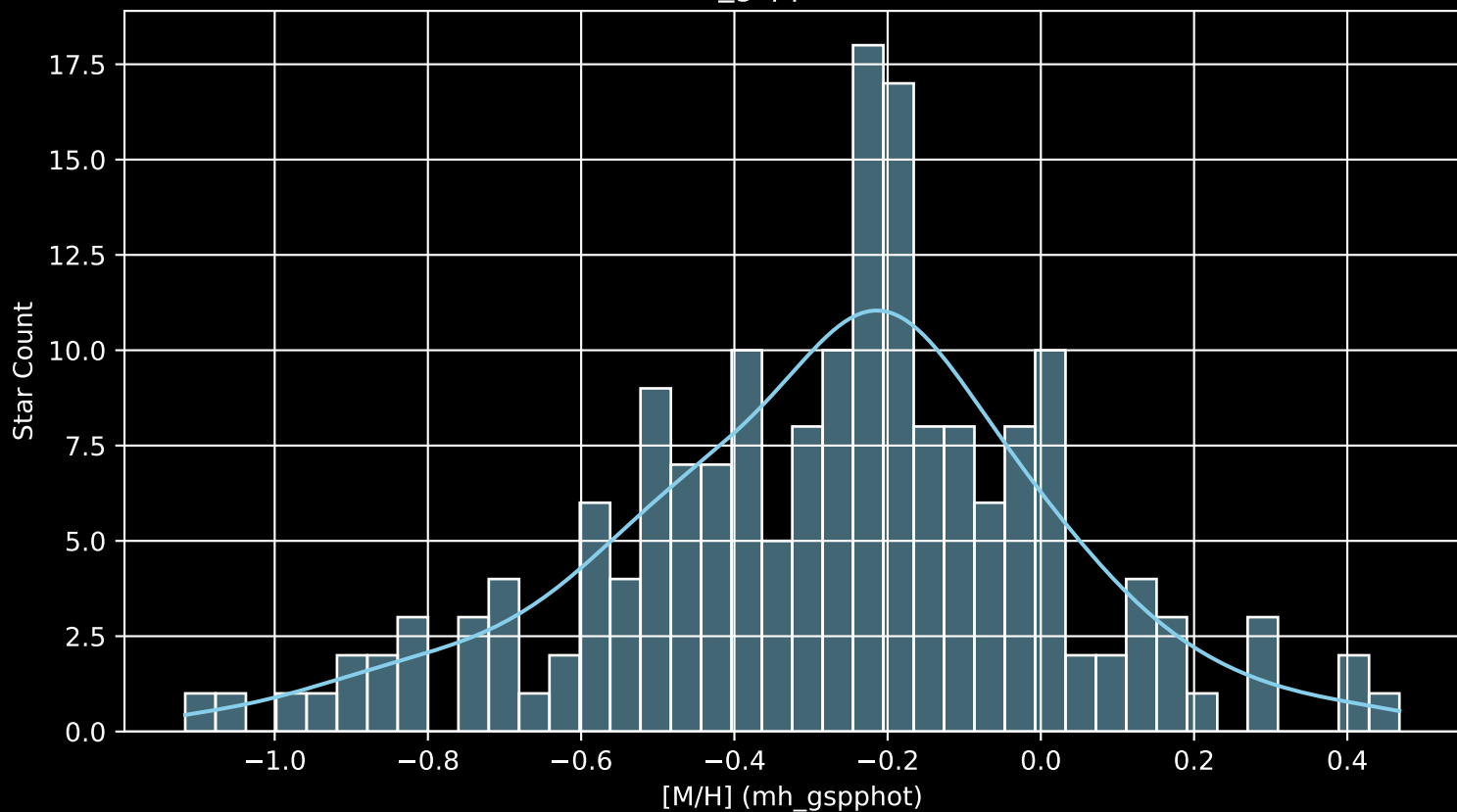
APOGEE DR17 Field: [201+37_MGA [M/H] (mh_gspphot) (n= 180)
