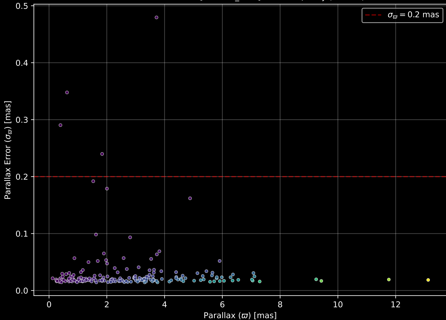
APOGEE DR17 Field: [201+37_MGA] Parallax Quality (n= 181)
