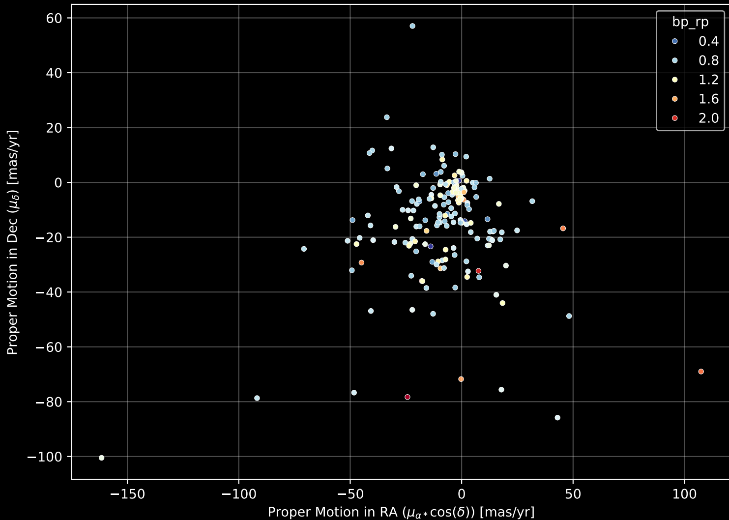
APOGEE DR17 Field: [201+37_MGA] Proper Motion Diagram (n= 181)
