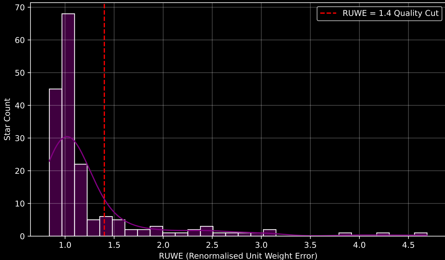
GAPOGEE DR17 Field [201+37_MGA] RUWE Distribution (n= 174)
