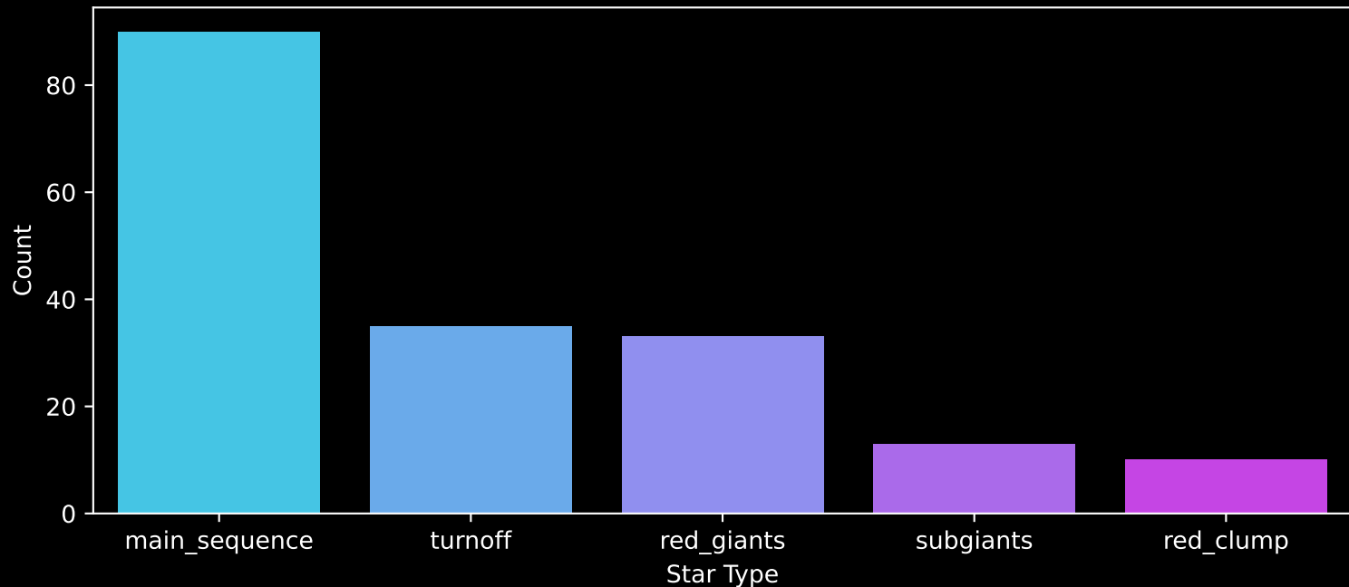
APOGEE DR17 Field: [201+37_MGA] Count plot of Star Type
