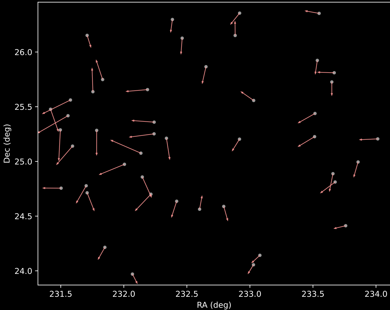
APOGEE DR17 Cluster 7 Proper Motion Vectors (n=45)
