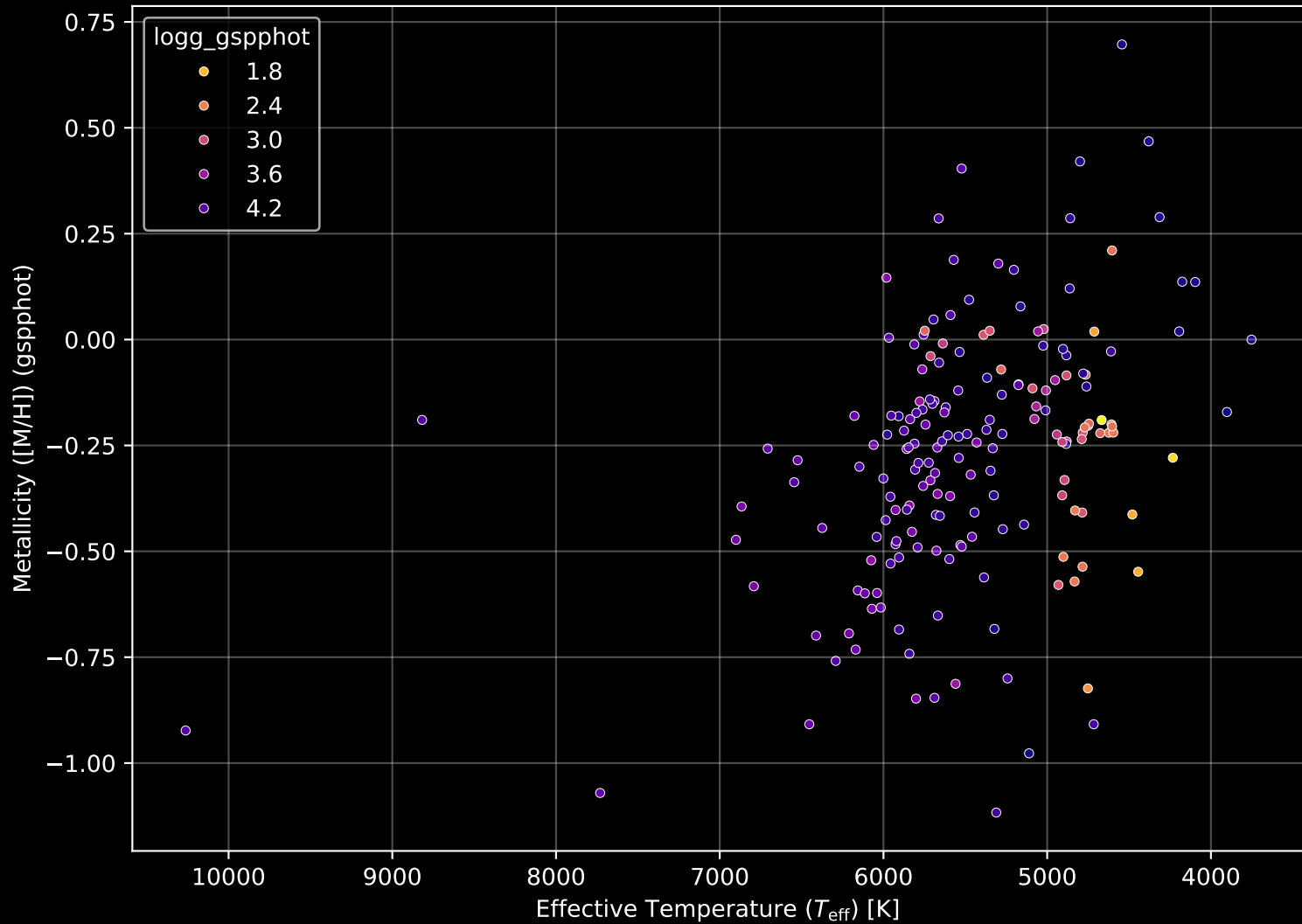
APOGEE DR17 Field: [201+37_MGA] Stellar Population Parameters (n= 181)
