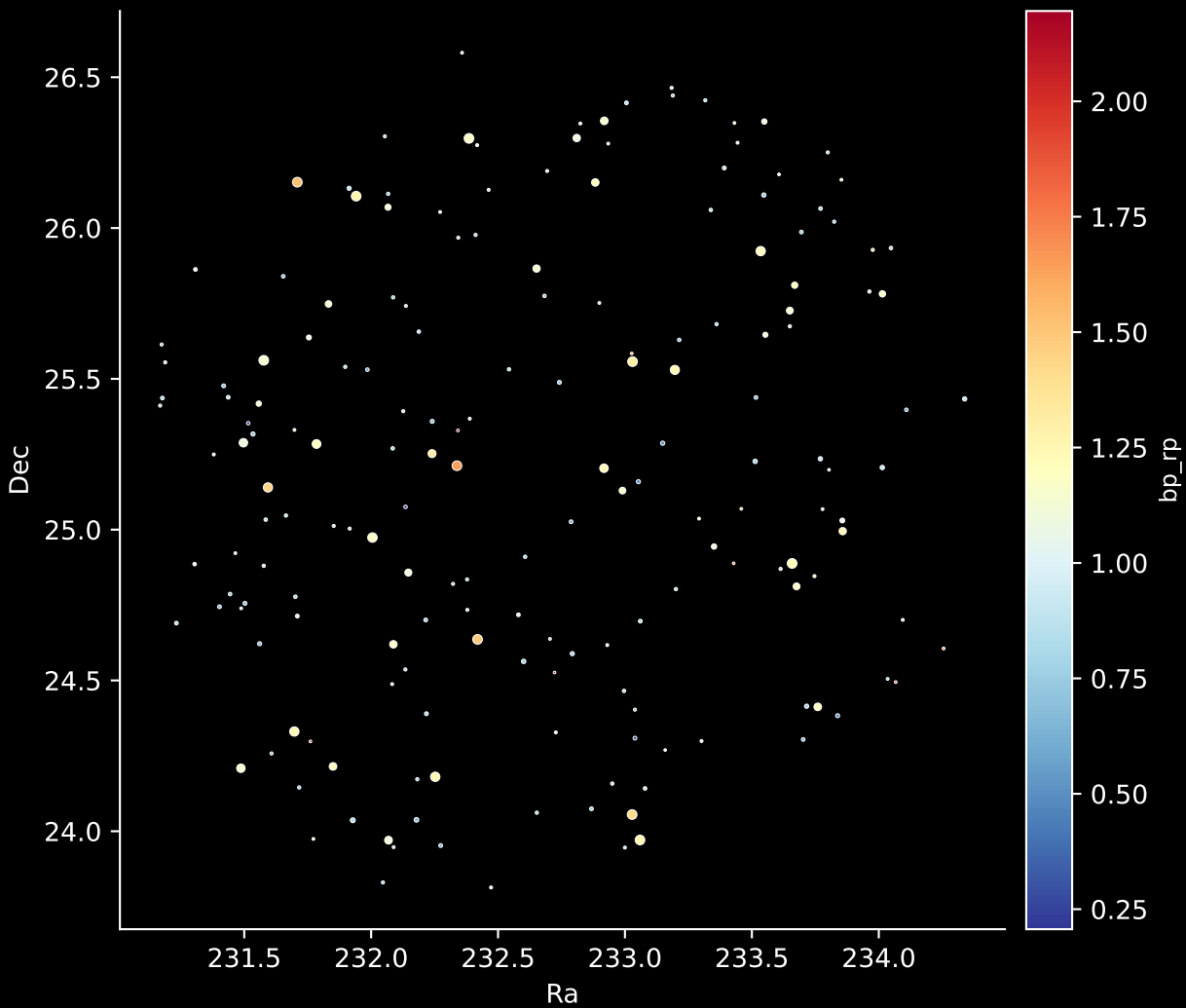
APOGEE DR17 Field: [201+37_MGA] Stars: 181
